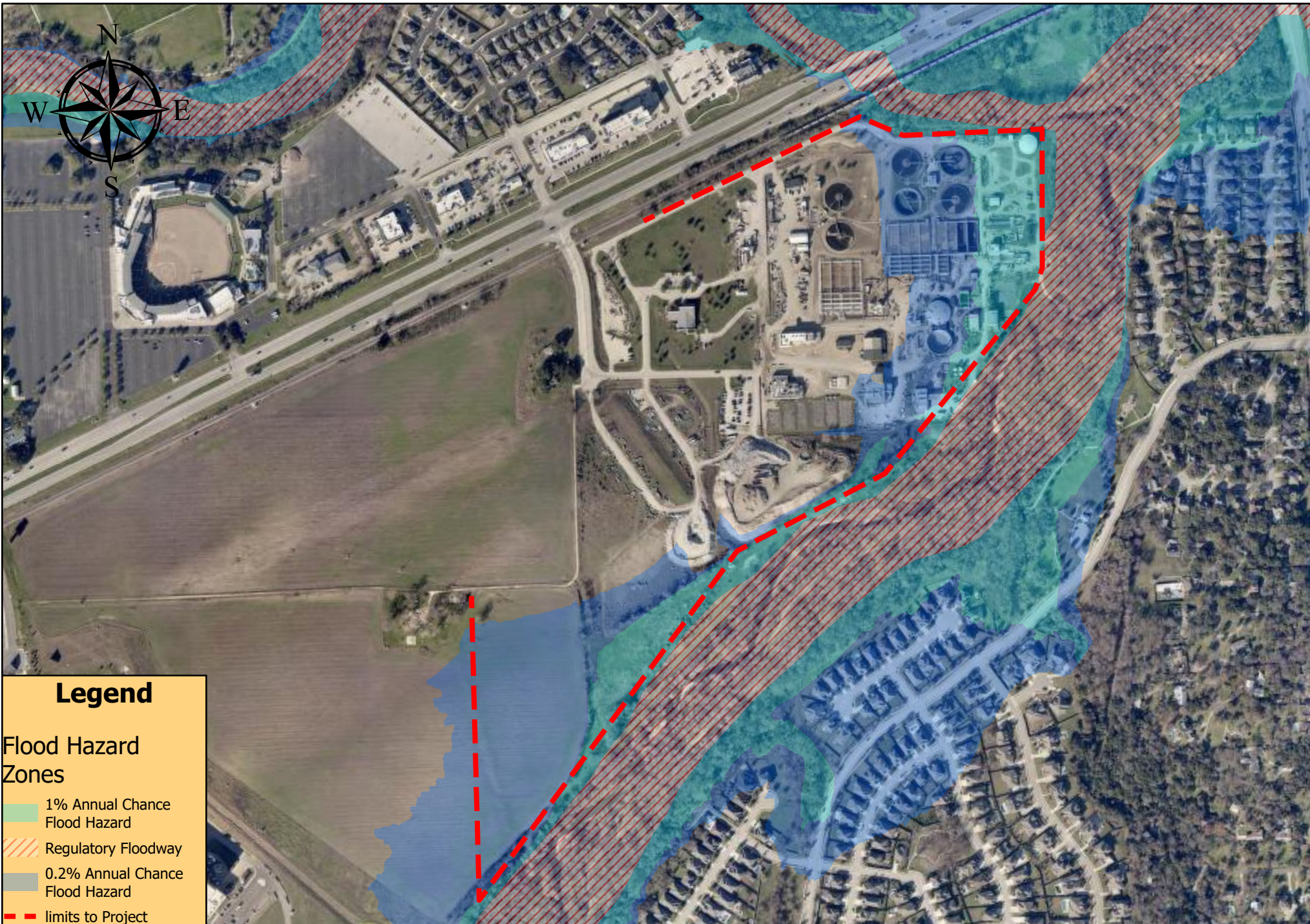
Brushy Creek East Wastewater Plant Floodwall Study
