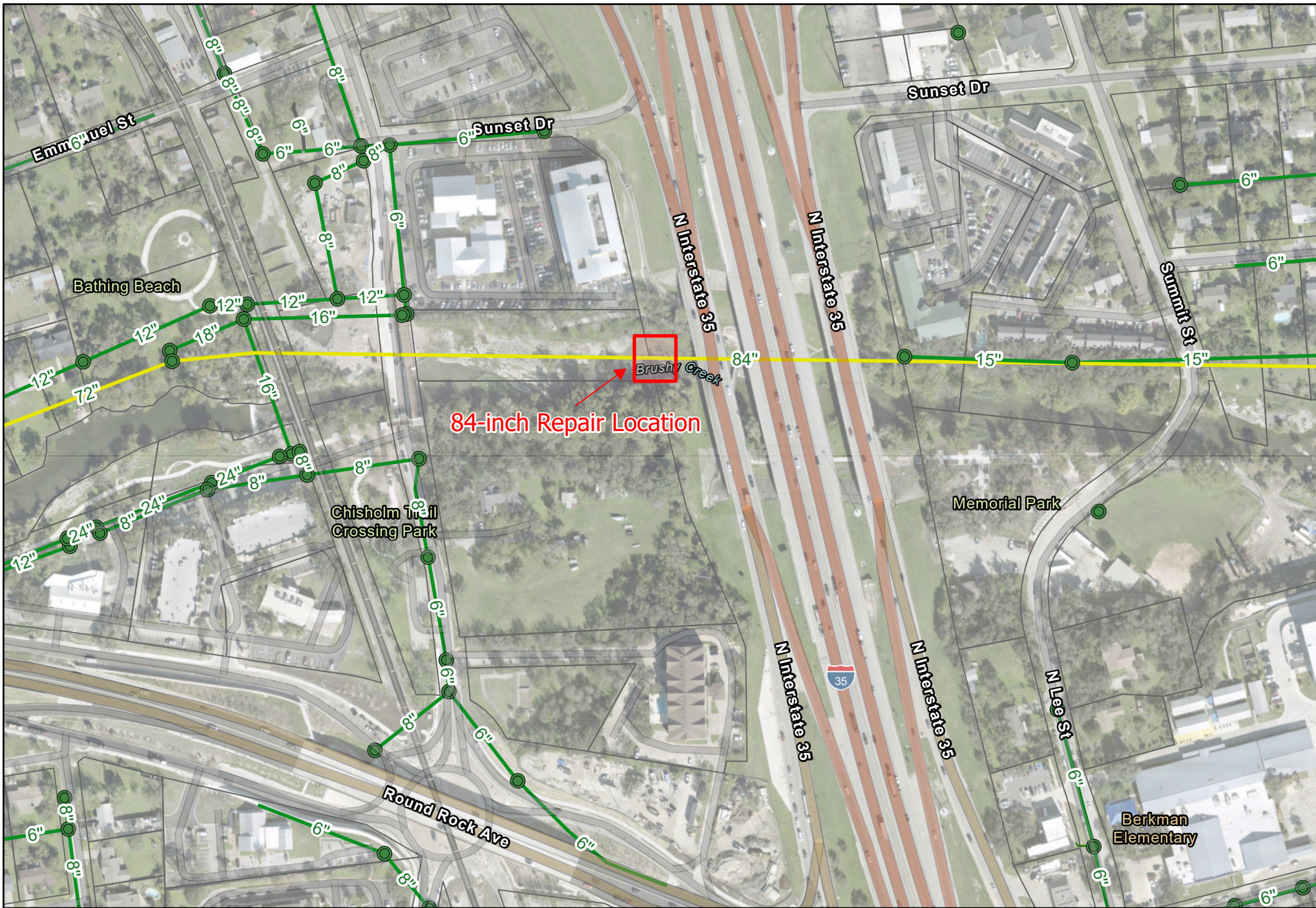
BCRWWS – 84” Tunnel Repair
