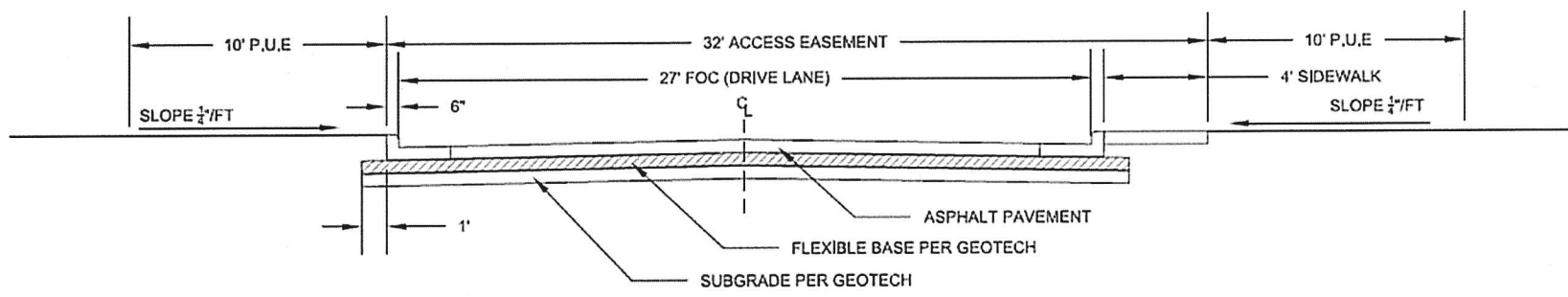
CURB AND GUTTER STREET SECTION
