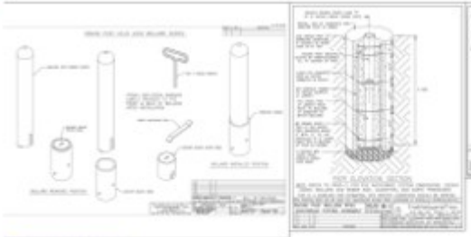
REMOVABLE BOLLARD
