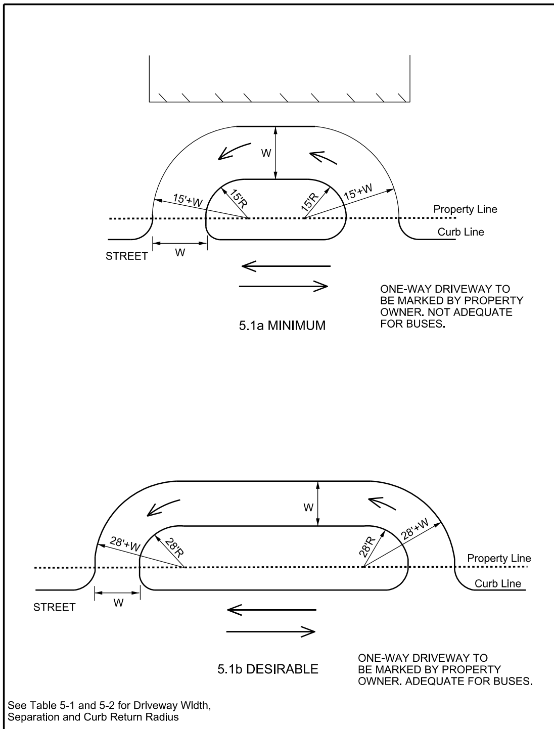
Figure 5.1 Design Criteria for Semicircular Drop-offs
