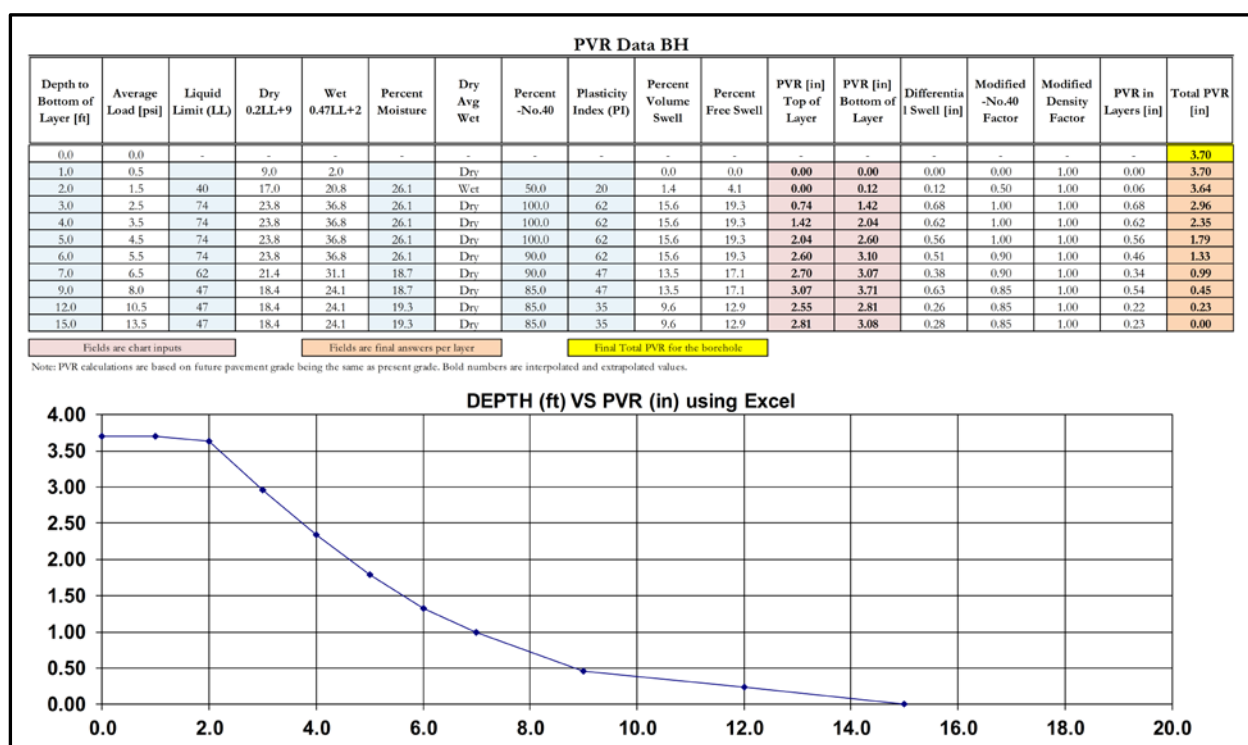
Figure 3-2. Example Calculation of PVR using TxDOT's Tex-124-E Calculation Spreadsheet (CAPEC 2016).
